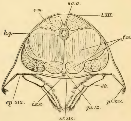
FIG. 36. — Astacus fluviatilis . — A transverse section through the nineteenth (fifth abdominal) somite ( \times 2 ). e.m. , extensor muscles; f.m. , flexor muscles; gn. 12. the fifth abdominal ganglion; h.g. , hind-gut; i.a.a. , inferior abdominal artery; s.a.a. , superior abdominal artery; pl. XIX. , pleura of the somite; st. XIX. , its sternum; t. XIX. , its tergum; ep. XIX. , its epimera; 19. , its appendages.
